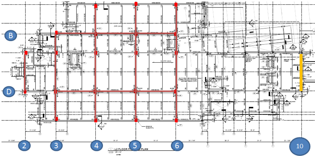
Figure 8: Location of Moment Frames (Red) and Braced Frame (Orange)
